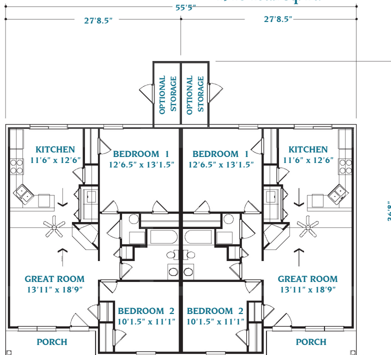
Duplex Plan 959 crawl 959 Per Unit 1918 Total Sq. Ft.
