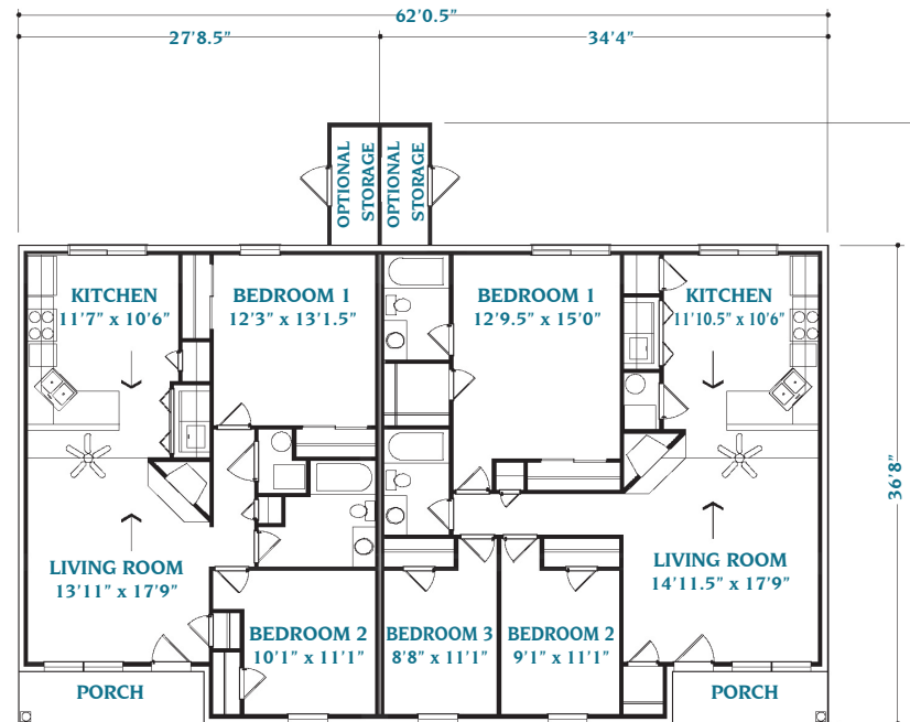
Duplex Plan 1211 959 Sq. Ft. Unit 1 1211 Sq. Ft. Unit 2 2170 Total Sq. Ft.
