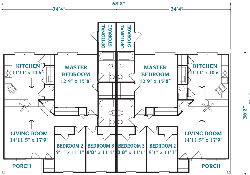
Duplex Plan 2428 1214 Per Unit 2428 Total Sq. Ft.
