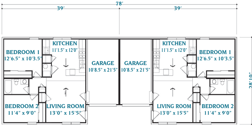
Duplex Plan 880 819 Sq. Ft. Per Unit 1638 Total Sq. Ft.
