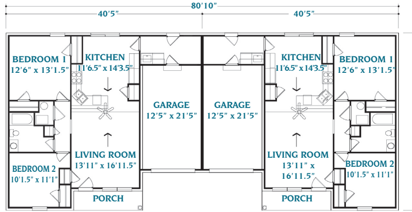
Duplex Plan 1058 1057 Sq. Ft. Per Unit 2114 Total Sq. Ft.
